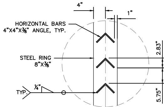
HORIZONTAL BAR DETAIL
