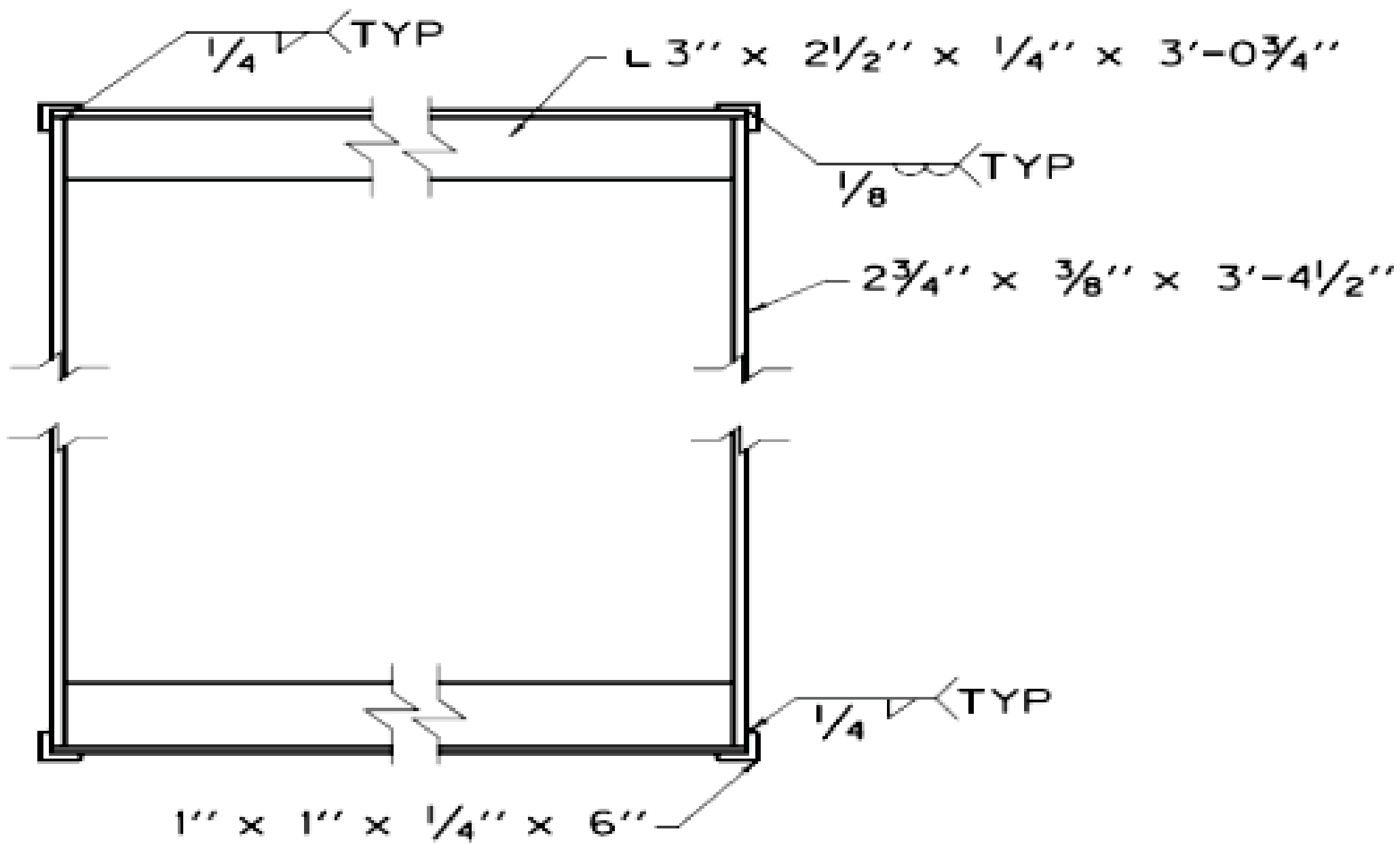
FRAME DETAIL
