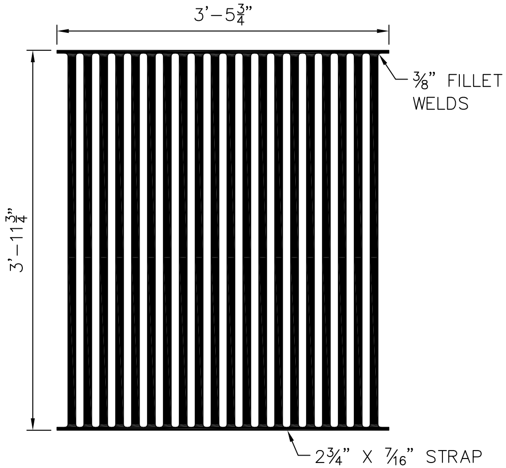
PLAN
