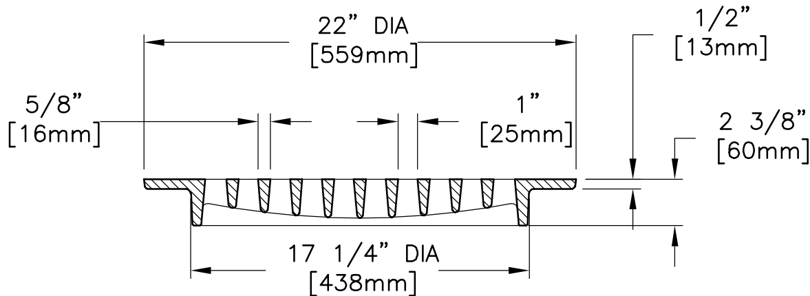
GRATE SECTION
