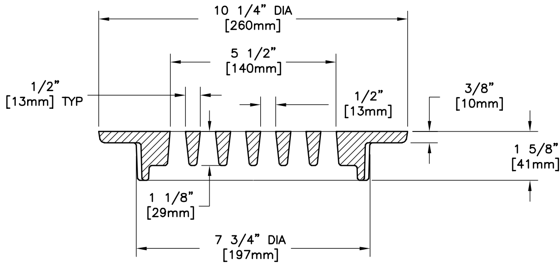
GRATE SECTION
