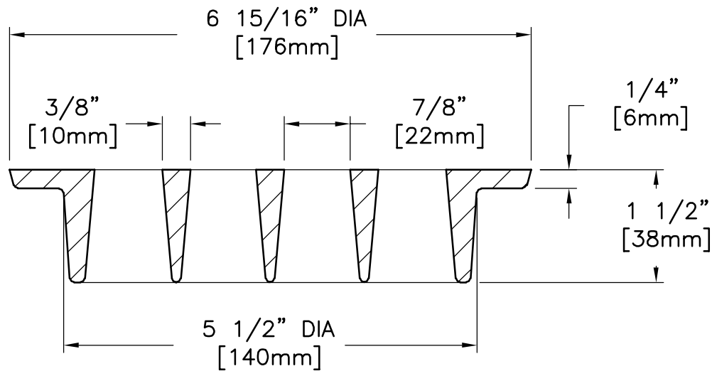
GRATE SECTION
