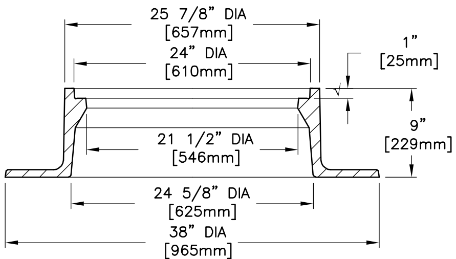
FRAME SECTION
