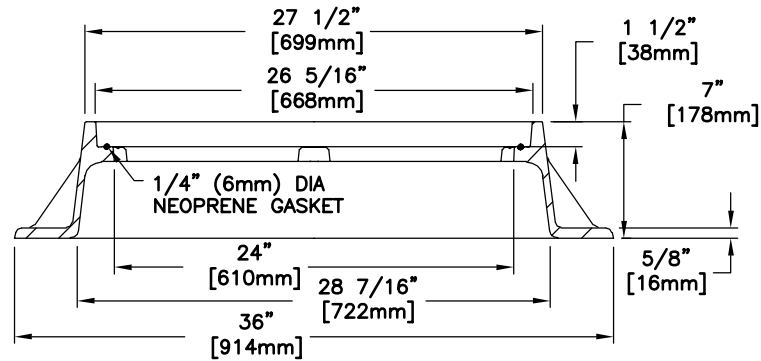
FRAME SECTION
