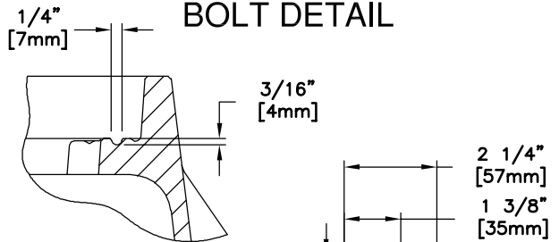
GROOVE DETAIL
