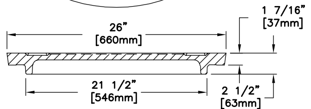
COVER SECTION
