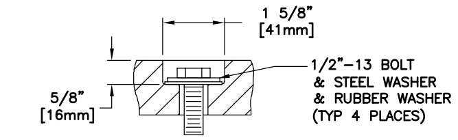
BOLT DETAIL
