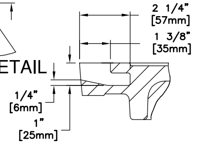
PICKHOLE DETAIL
