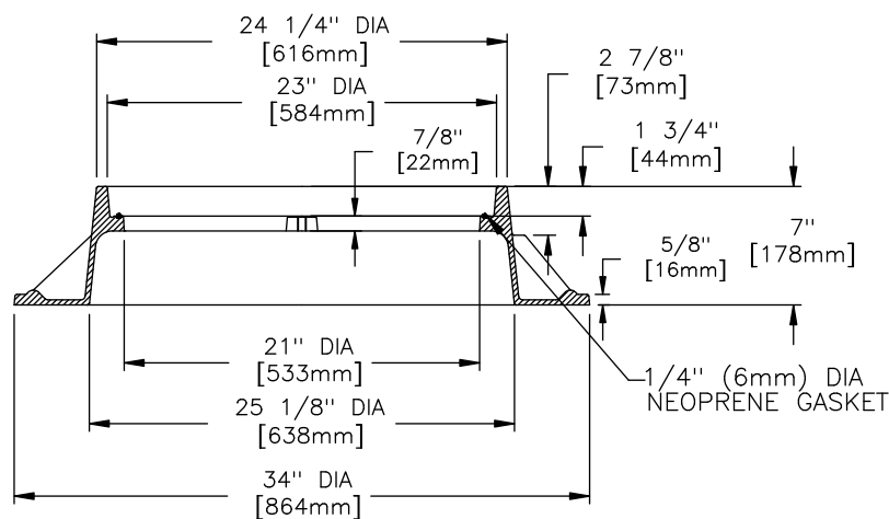
FRAME SECTION
