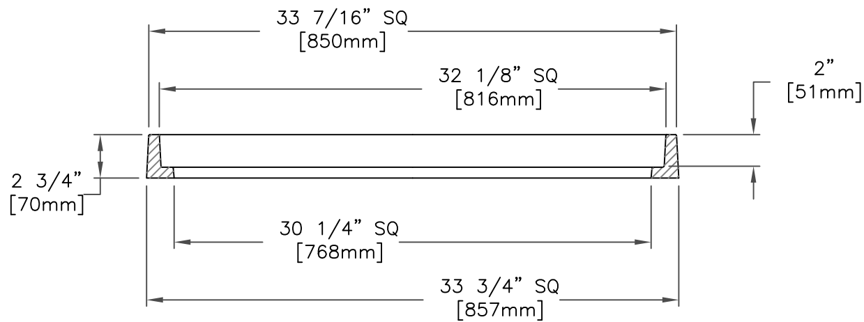
FRAME SECTION
