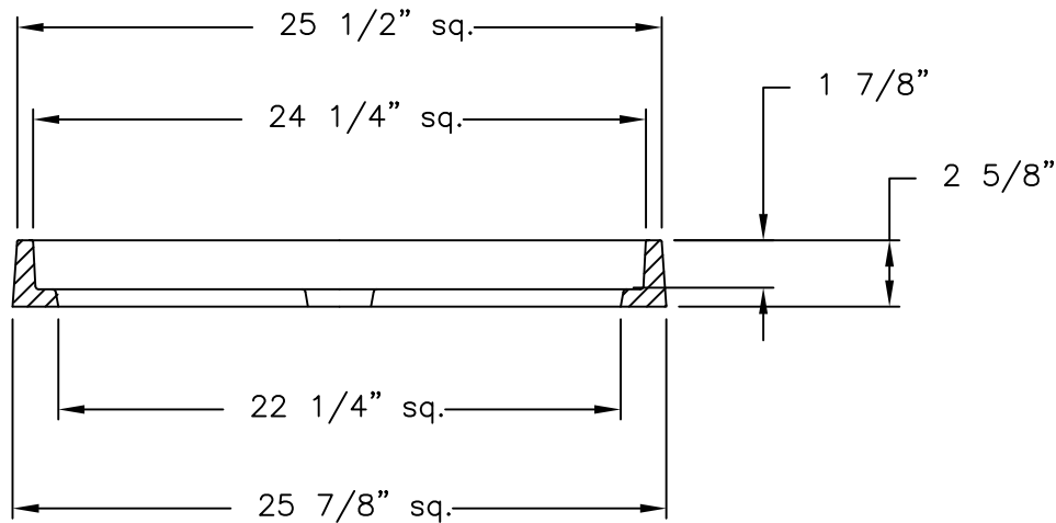
FRAME SECTION
