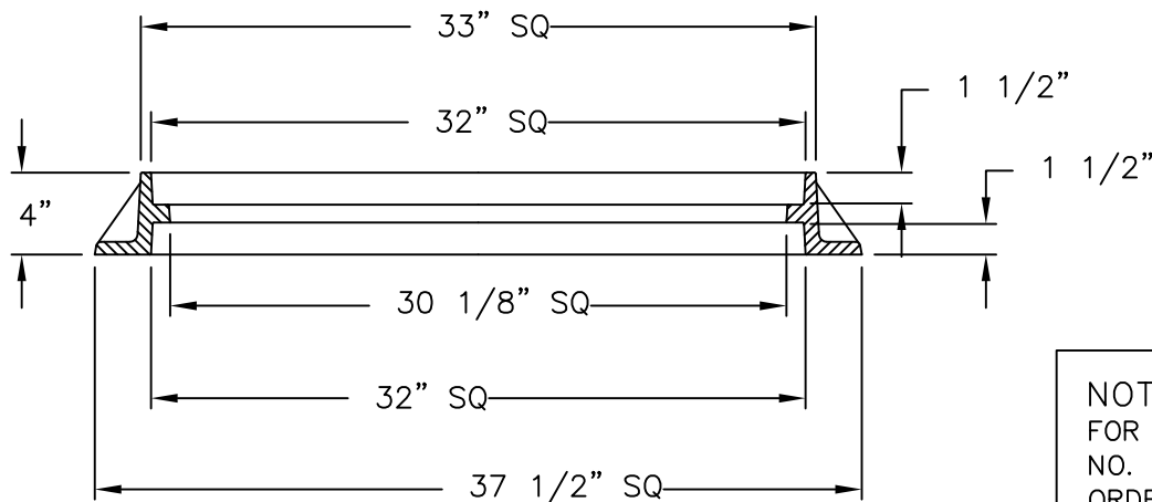
FRAME SECTION
