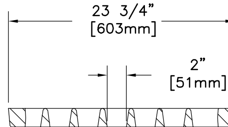
GRATE SECTION
