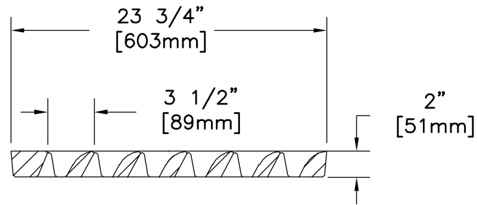
GRATE SECTION
